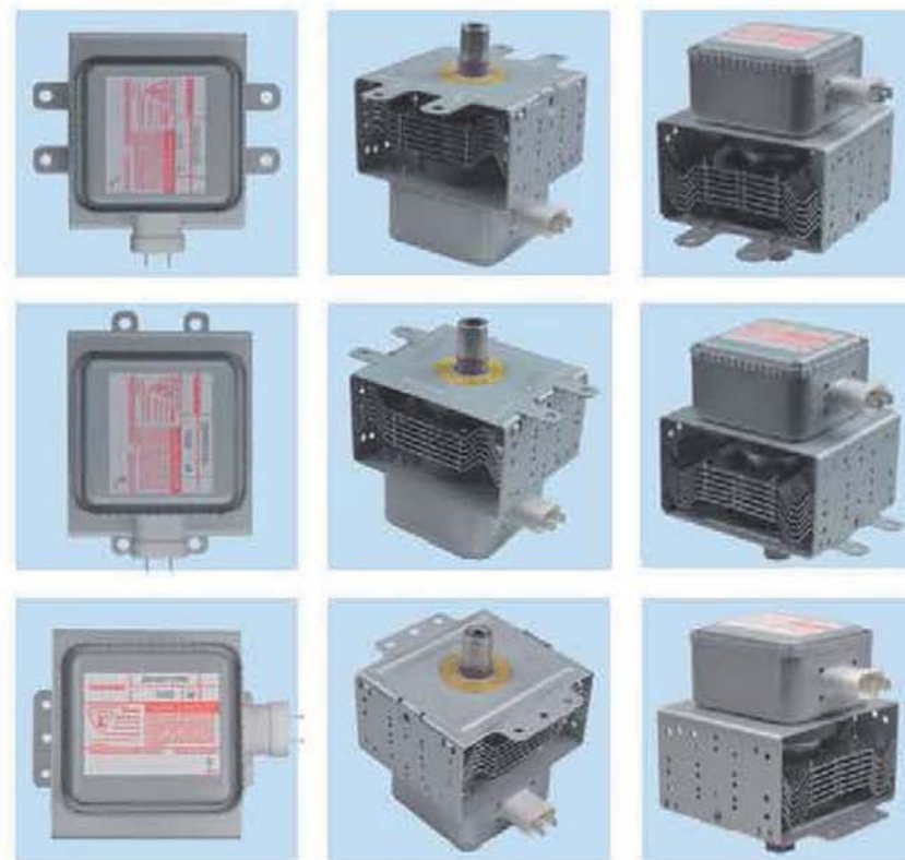
Toshiba air-cooled magnetron, models include: 2m248k, 2m248j, 2m248h, 2m303h, etc
